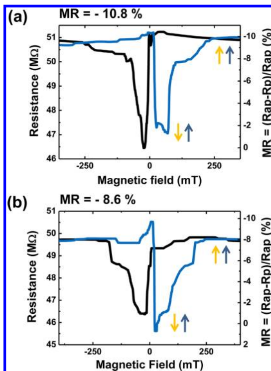
Figure 4. Spin transport through the Ni/graphene/Al 2 O 3 /Co junction at 1.4 K (a) A negative magnetoresistance \text{MR} = -10.8\% is measured (applied DC bias 100 mV). (b) Magnetoresistance measured at -100 mV.
